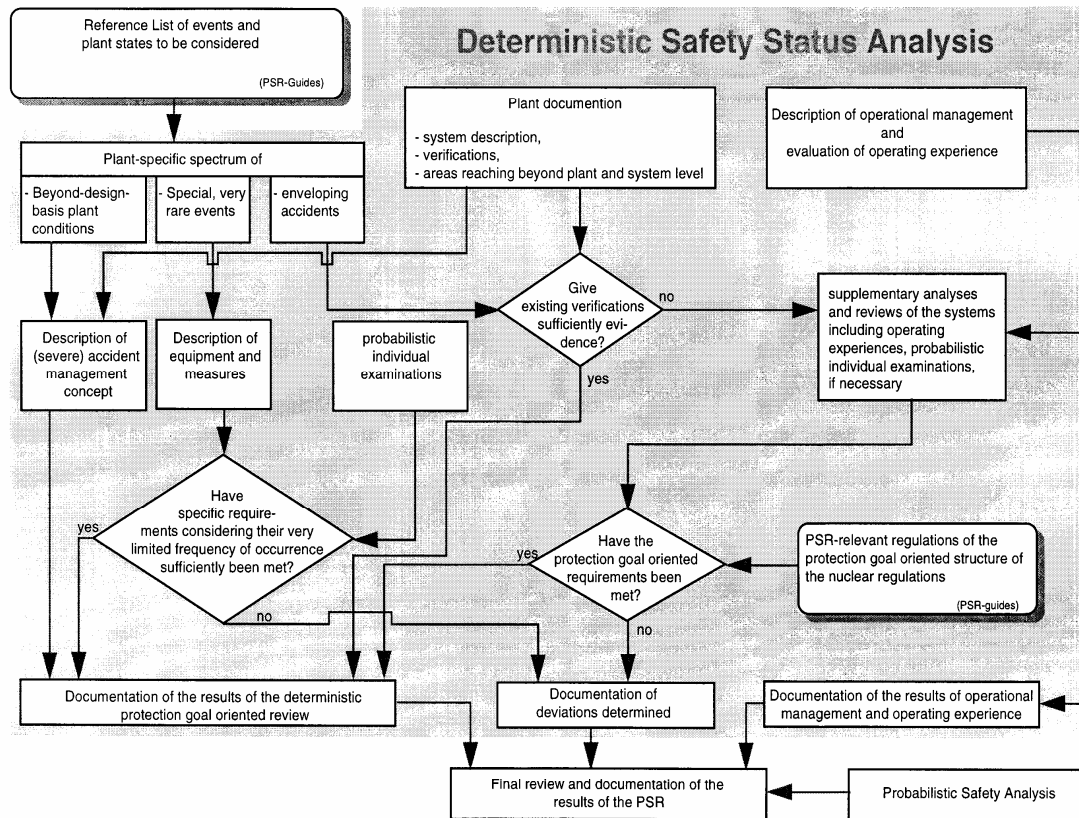
Fig. 2: Procedure of deterministic safety status analysis
