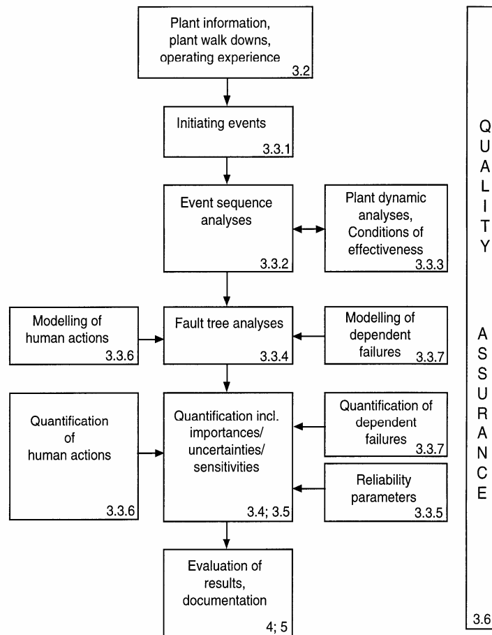
Fig. 1: Flow chart of the Probabilistic Safety Analysis (PSA) within the framework of the Periodic Safety Review (including references to the respective sections in the present guide)
